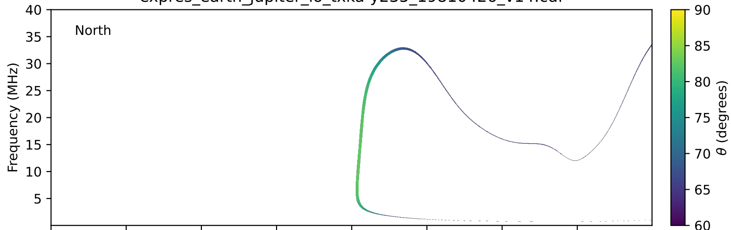
expres_earth_jupiter_io_txka-y235_19810426_v14.cdf
