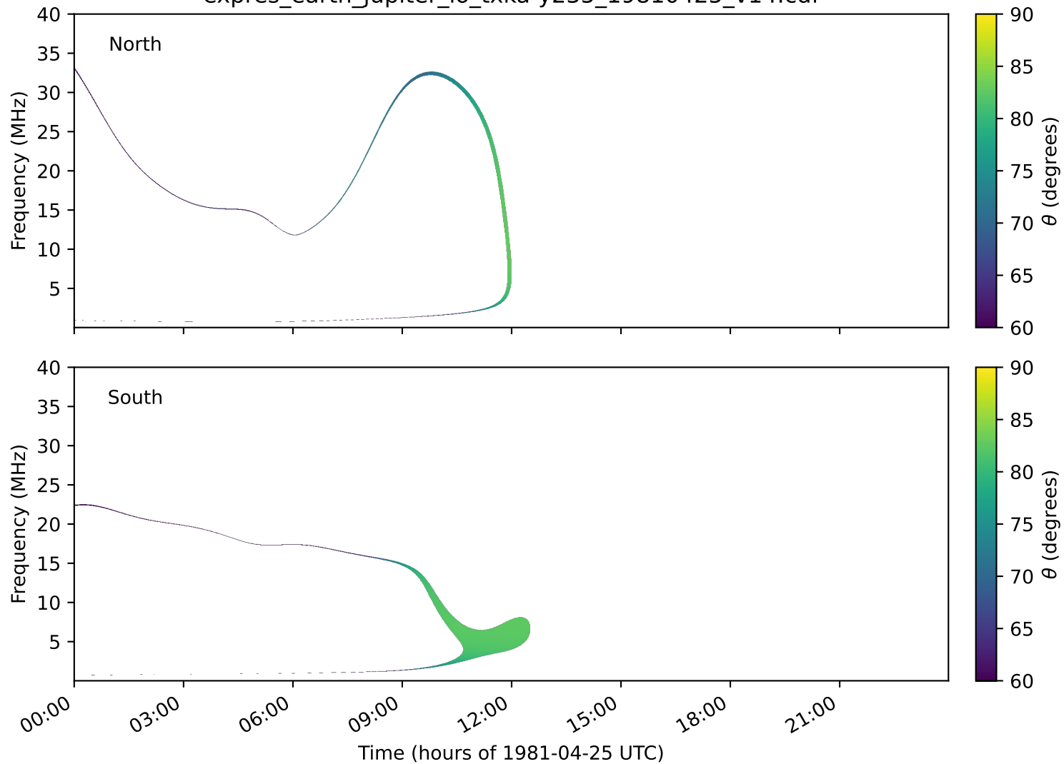
expres_earth_jupiter_io_txka-y235_19810425_v14.cdf
