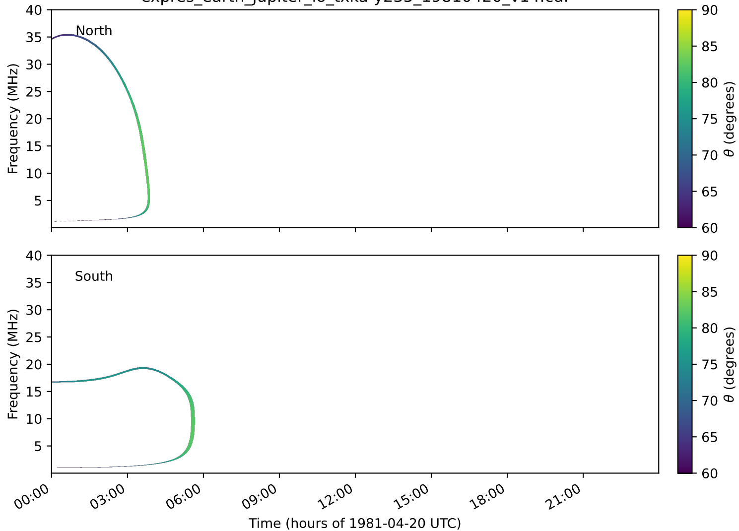
expres_earth_jupiter_io_txka-y235_19810420_v14.cdf
