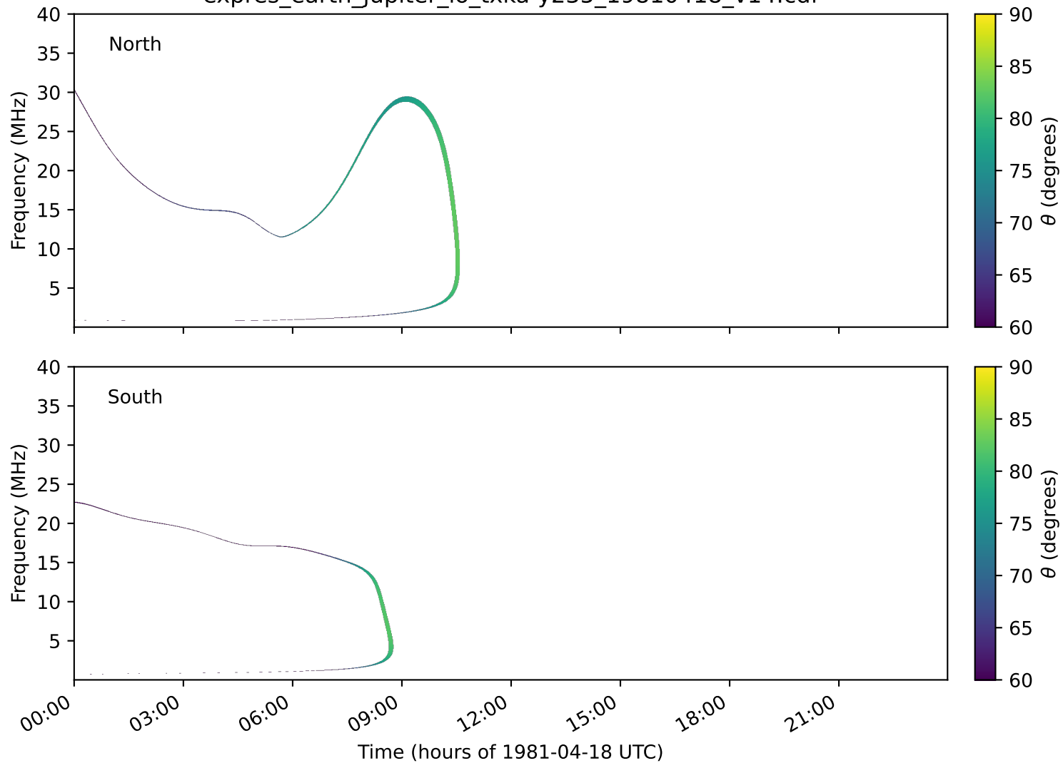
expres_earth_jupiter_io_txka-y235_19810418_v14.cdf
