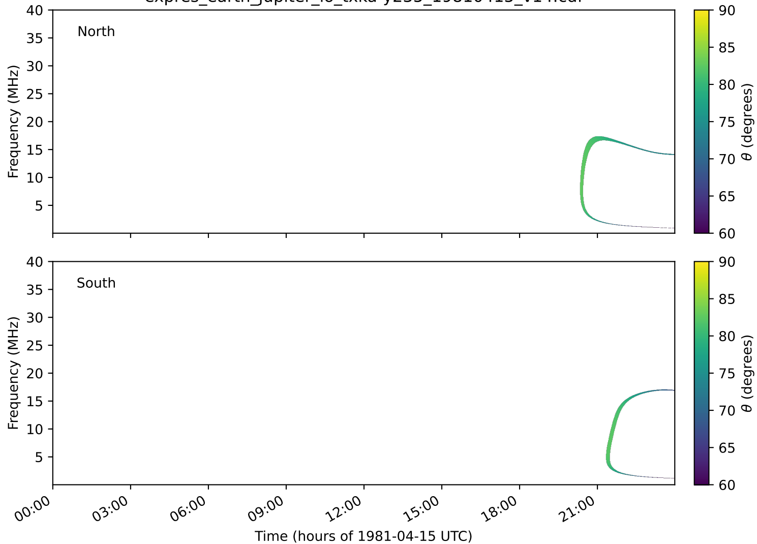
expres_earth_jupiter_io_txka-y235_19810415_v14.cdf
