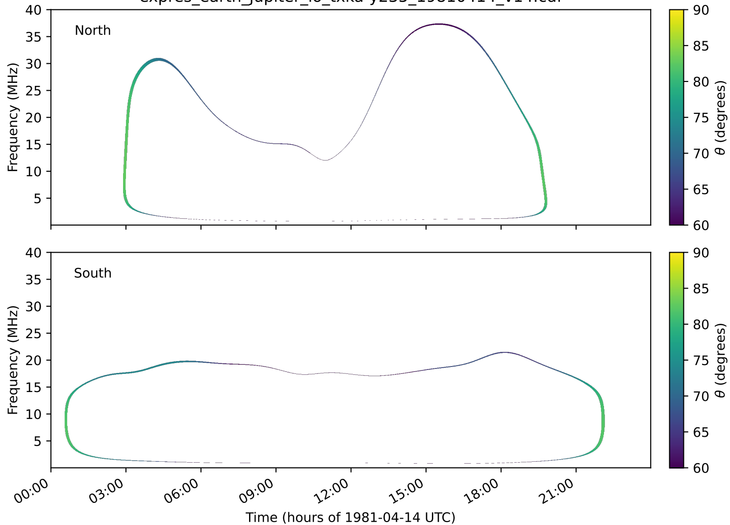
expres_earth_jupiter_io_txka-y235_19810414_v14.cdf
