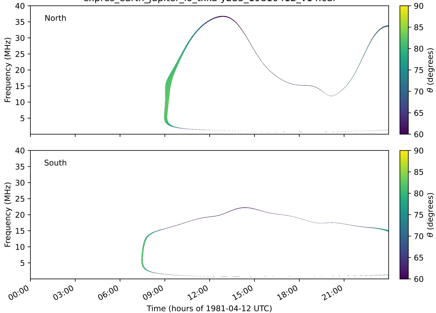
expres_earth_jupiter_io_txka-y235_19810412_v14.cdf
