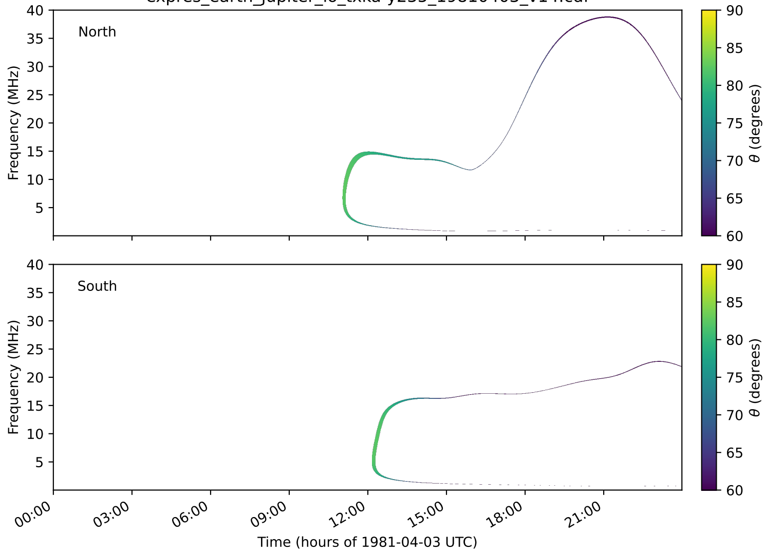
expres_earth_jupiter_io_txka-y235_19810403_v14.cdf
