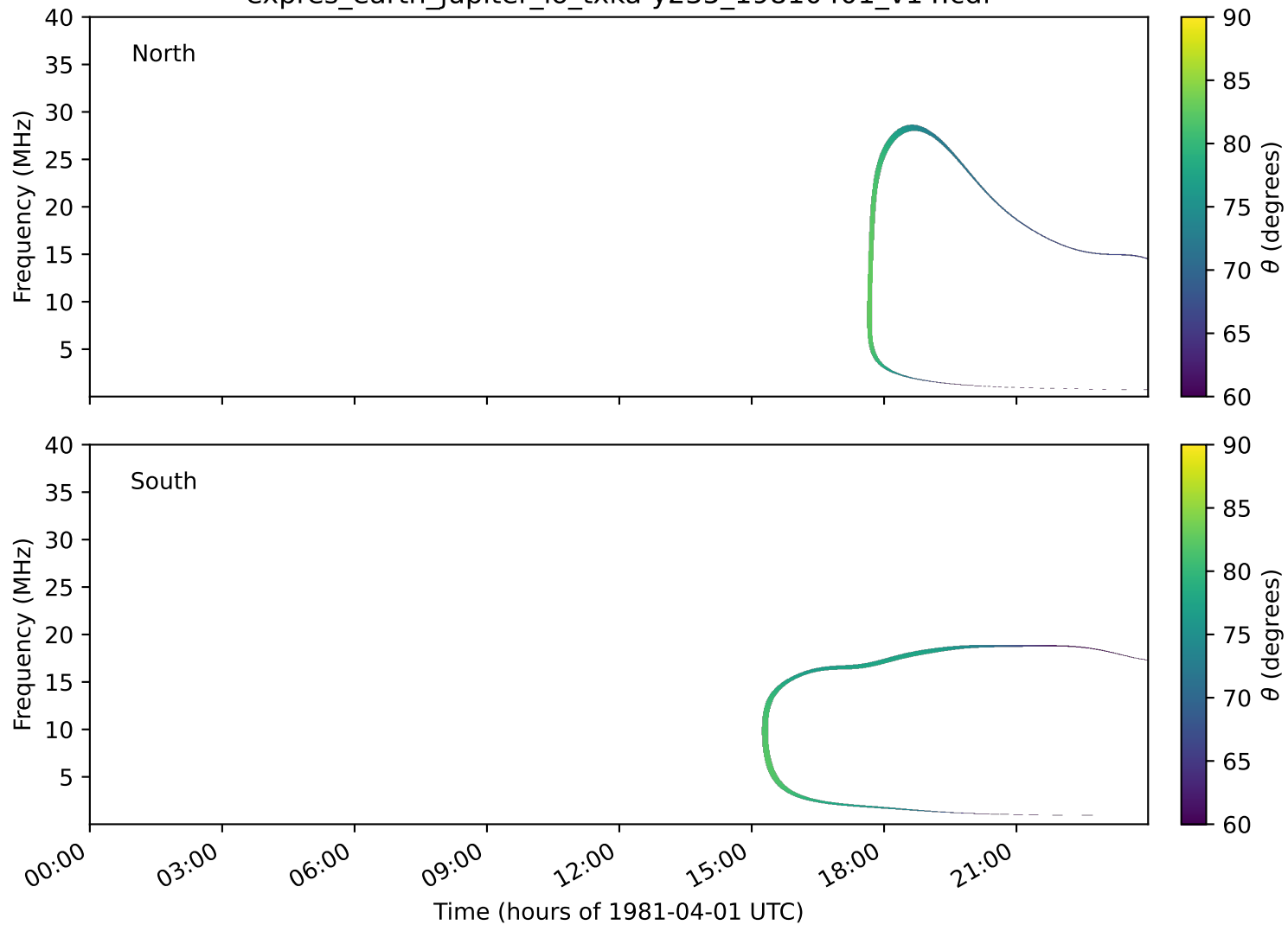
expres_earth_jupiter_io_txka-y235_19810401_v14.cdf
