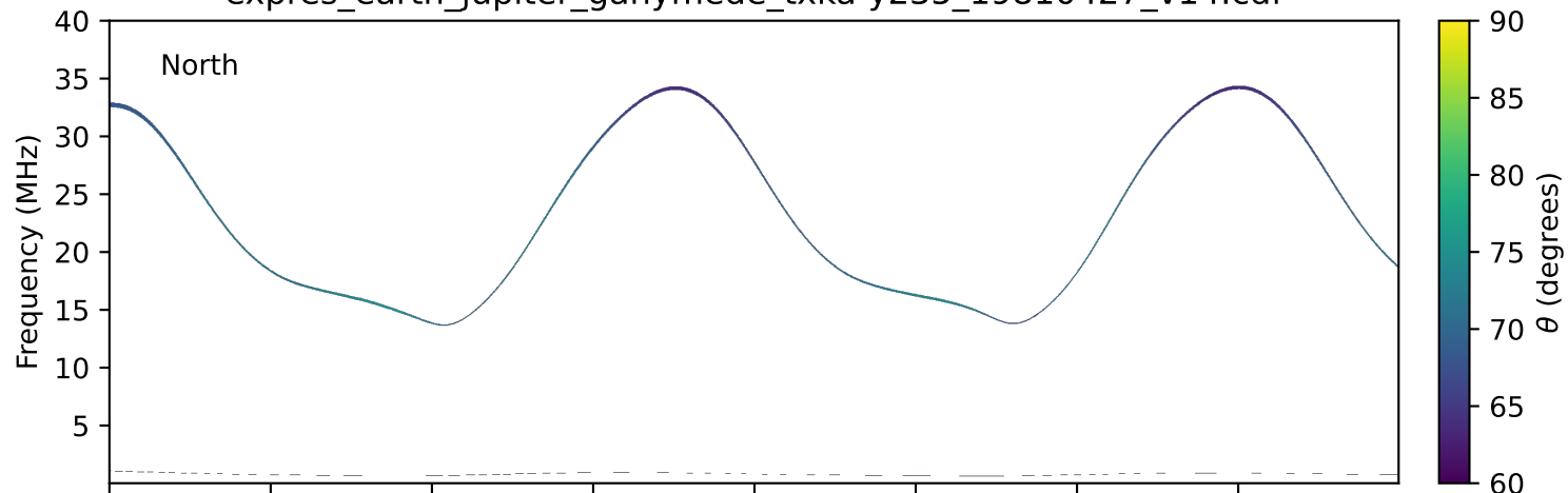
expres_earth_jupiter_ganymede_txka-y235_19810427_v14.cdf
