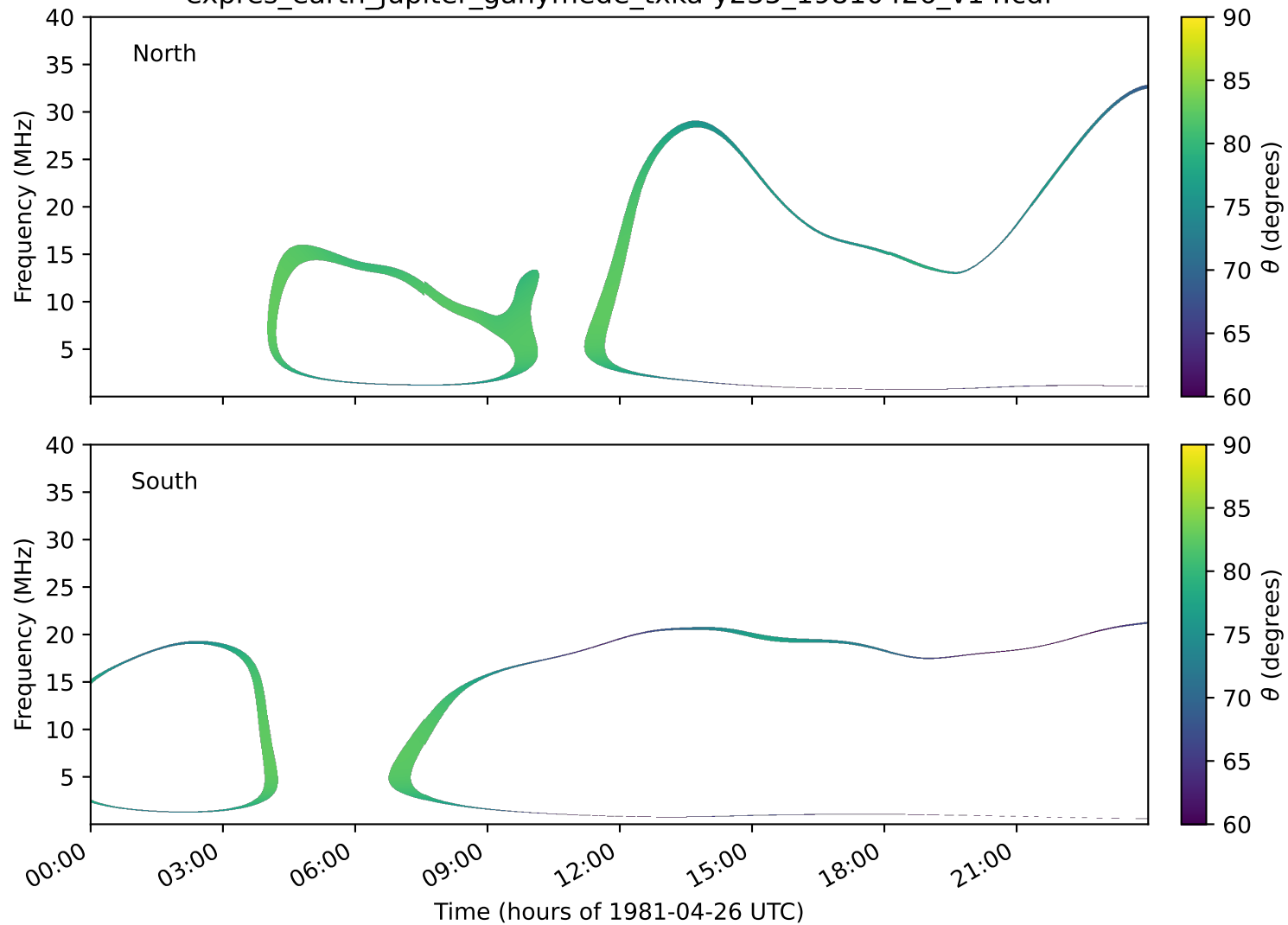
expres_earth_jupiter_ganymede_txka-y235_19810426_v14.cdf
