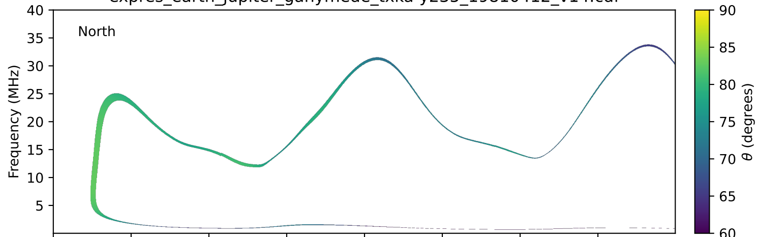
expres_earth_jupiter_ganymede_txka-y235_19810412_v14.cdf
