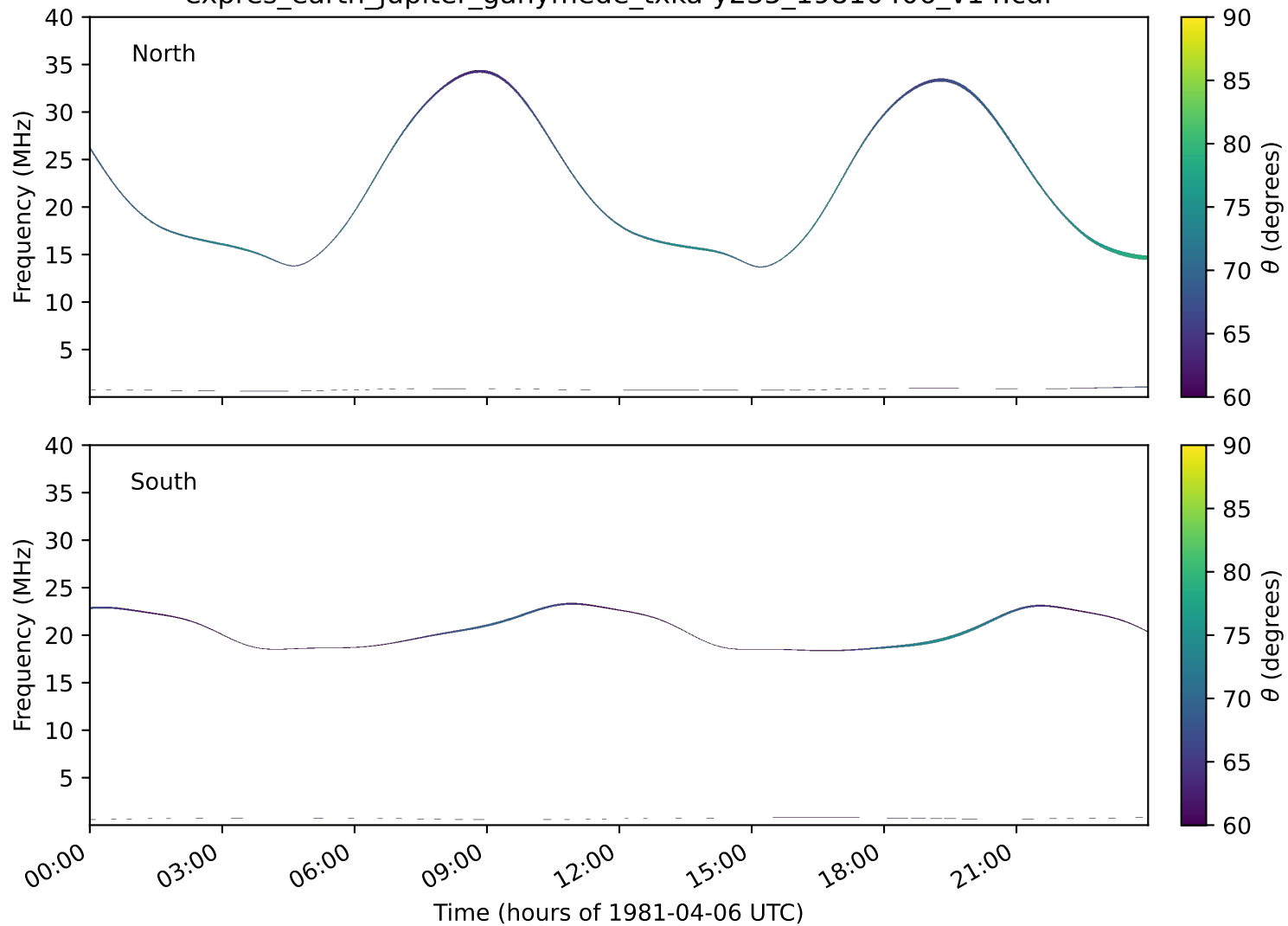
expres_earth_jupiter_ganymede_txka-y235_19810406_v14.cdf
