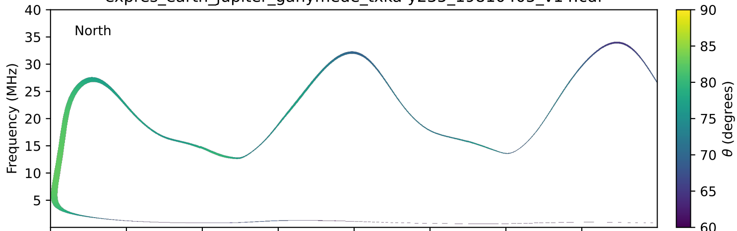
expres_earth_jupiter_ganymede_txka-y235_19810405_v14.cdf
