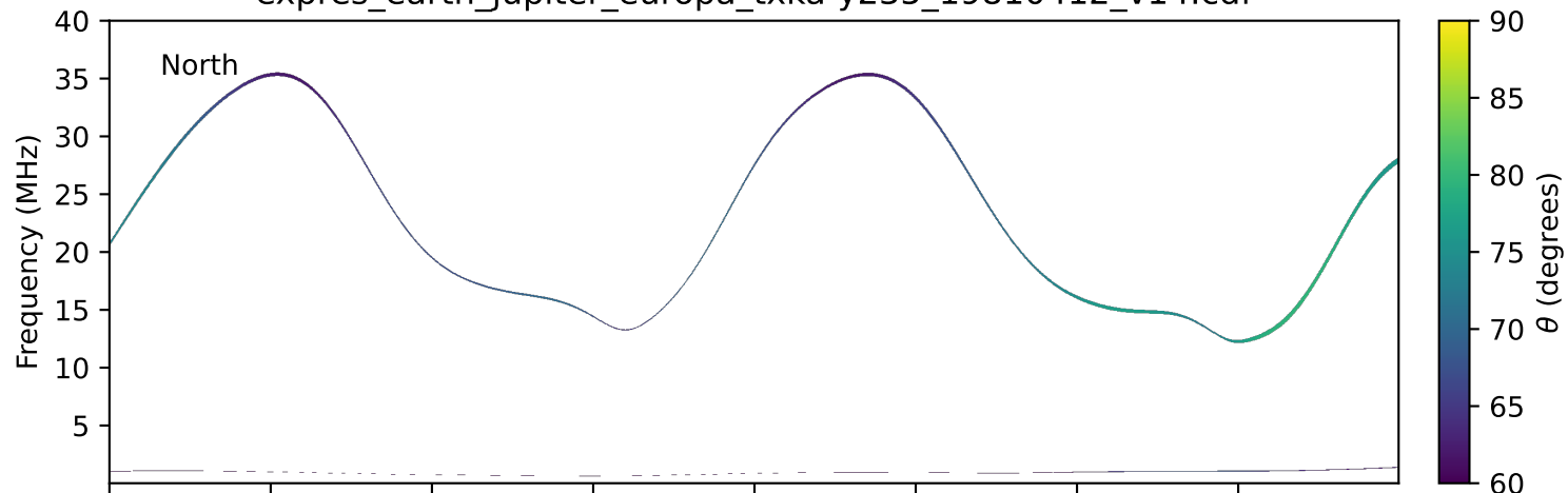
expres_earth_jupiter_europa_txka-y235_19810412_v14.cdf
