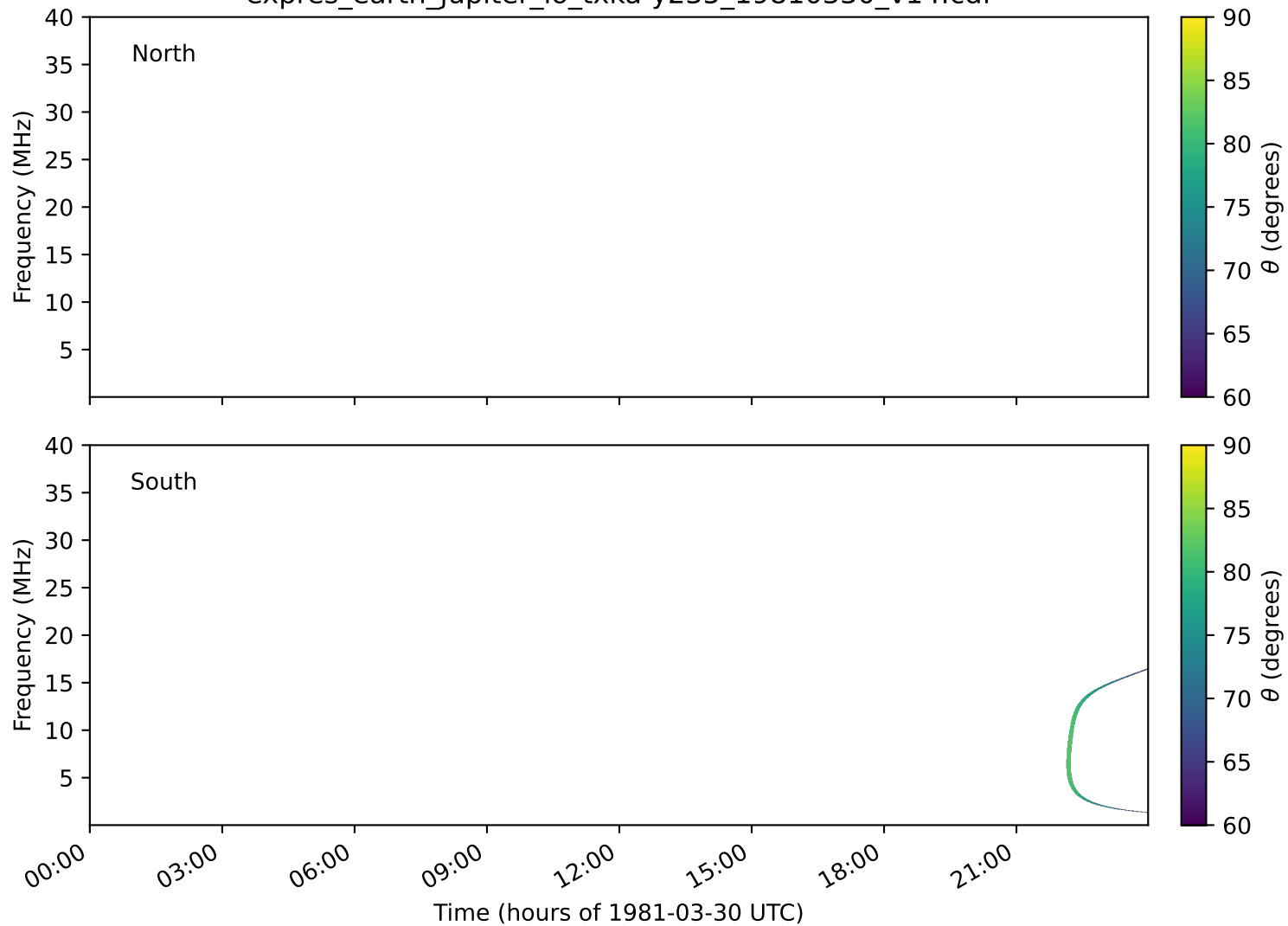
expres_earth_jupiter_io_txka-y235_19810330_v14.cdf
