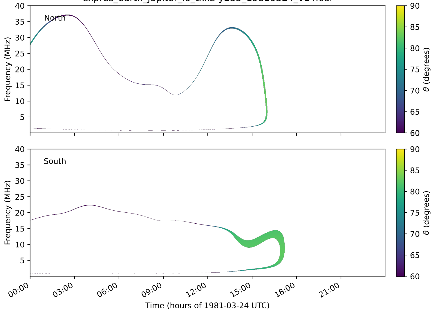
expres_earth_jupiter_io_txka-y235_19810324_v14.cdf
