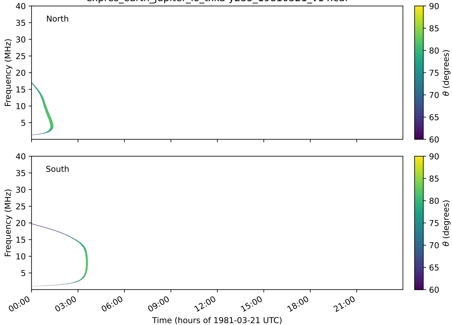
expres_earth_jupiter_io_txka-y235_19810321_v14.cdf
