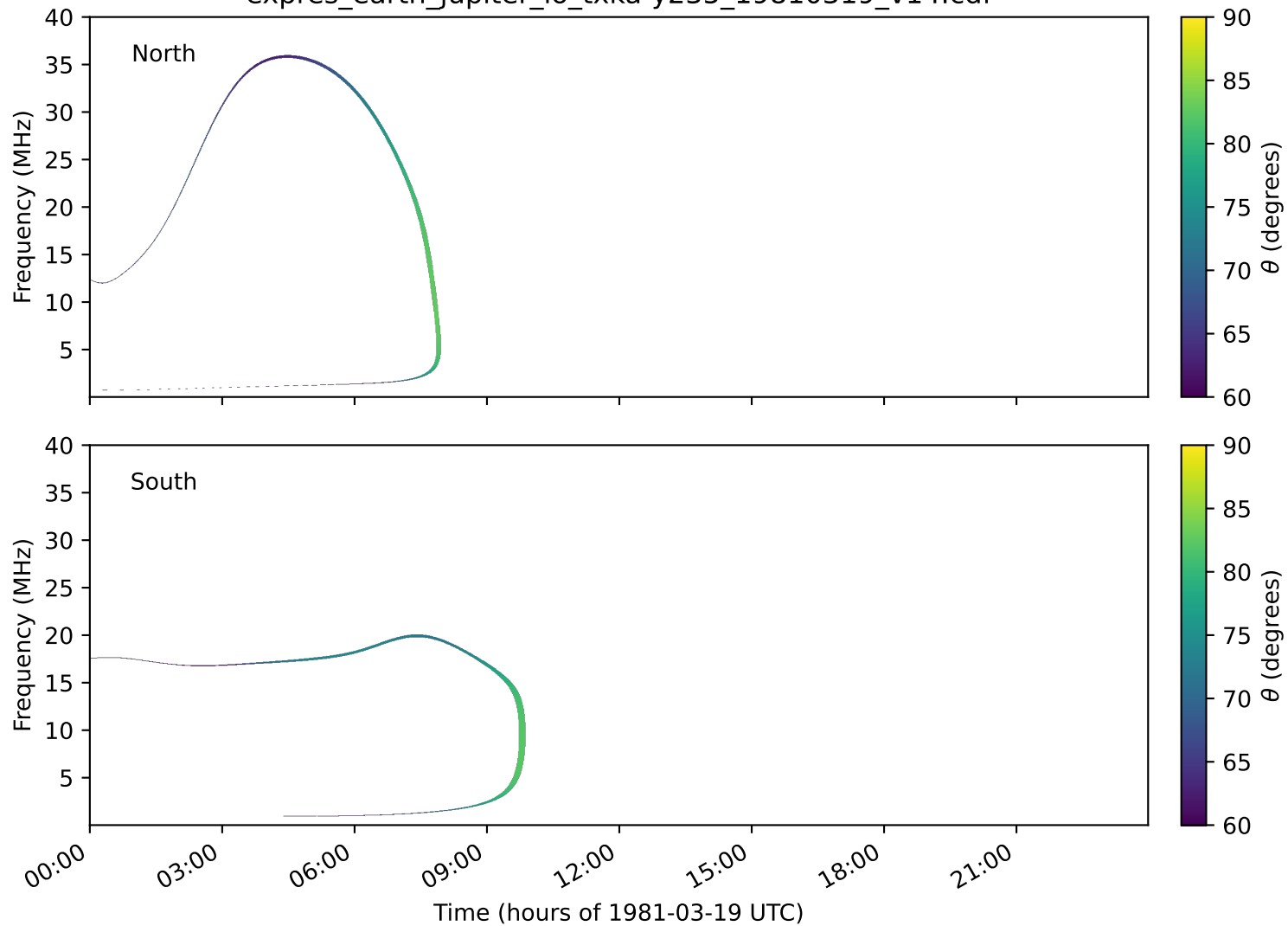
expres_earth_jupiter_io_txka-y235_19810319_v14.cdf
