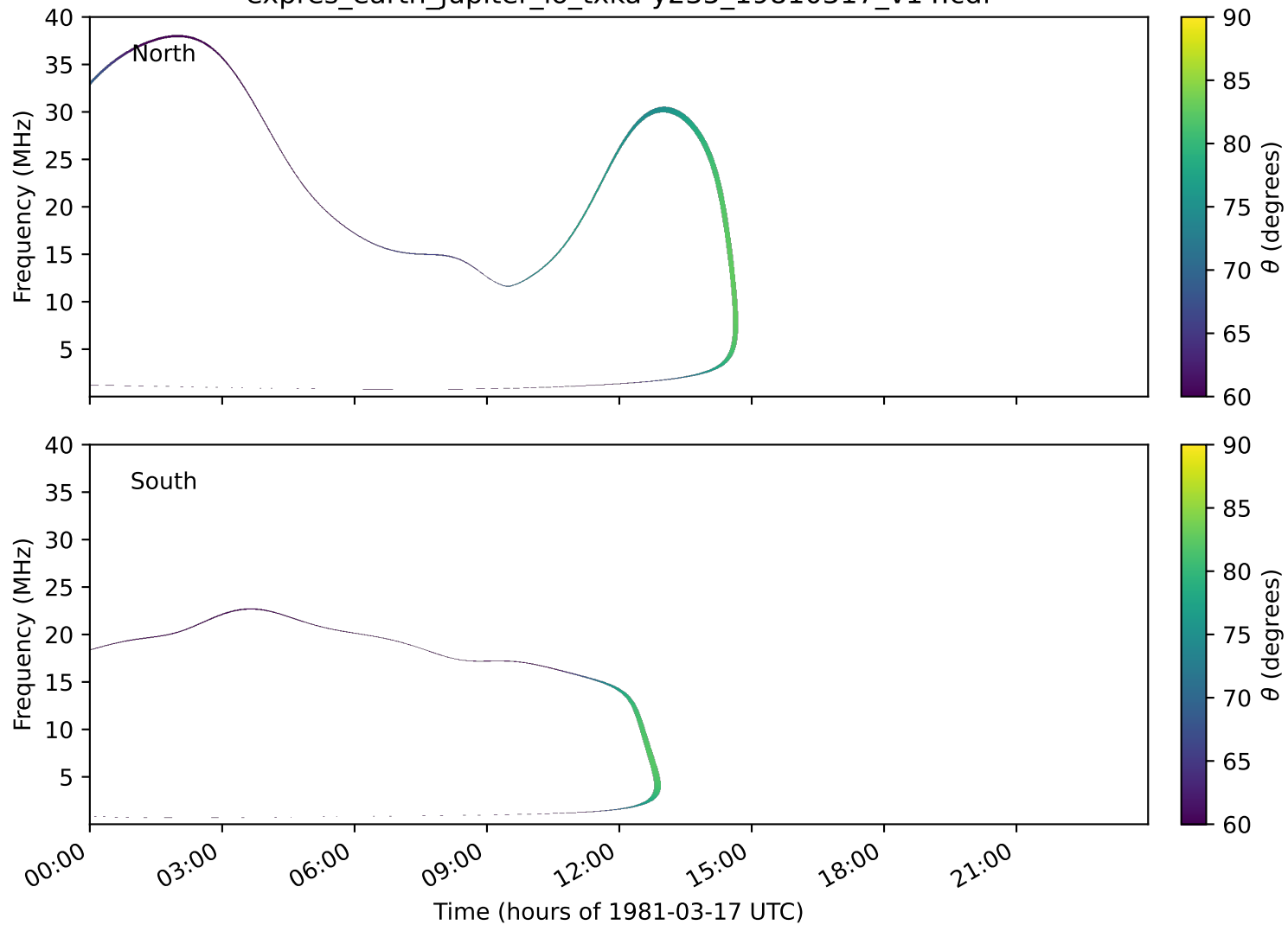
expres_earth_jupiter_io_txka-y235_19810317_v14.cdf
