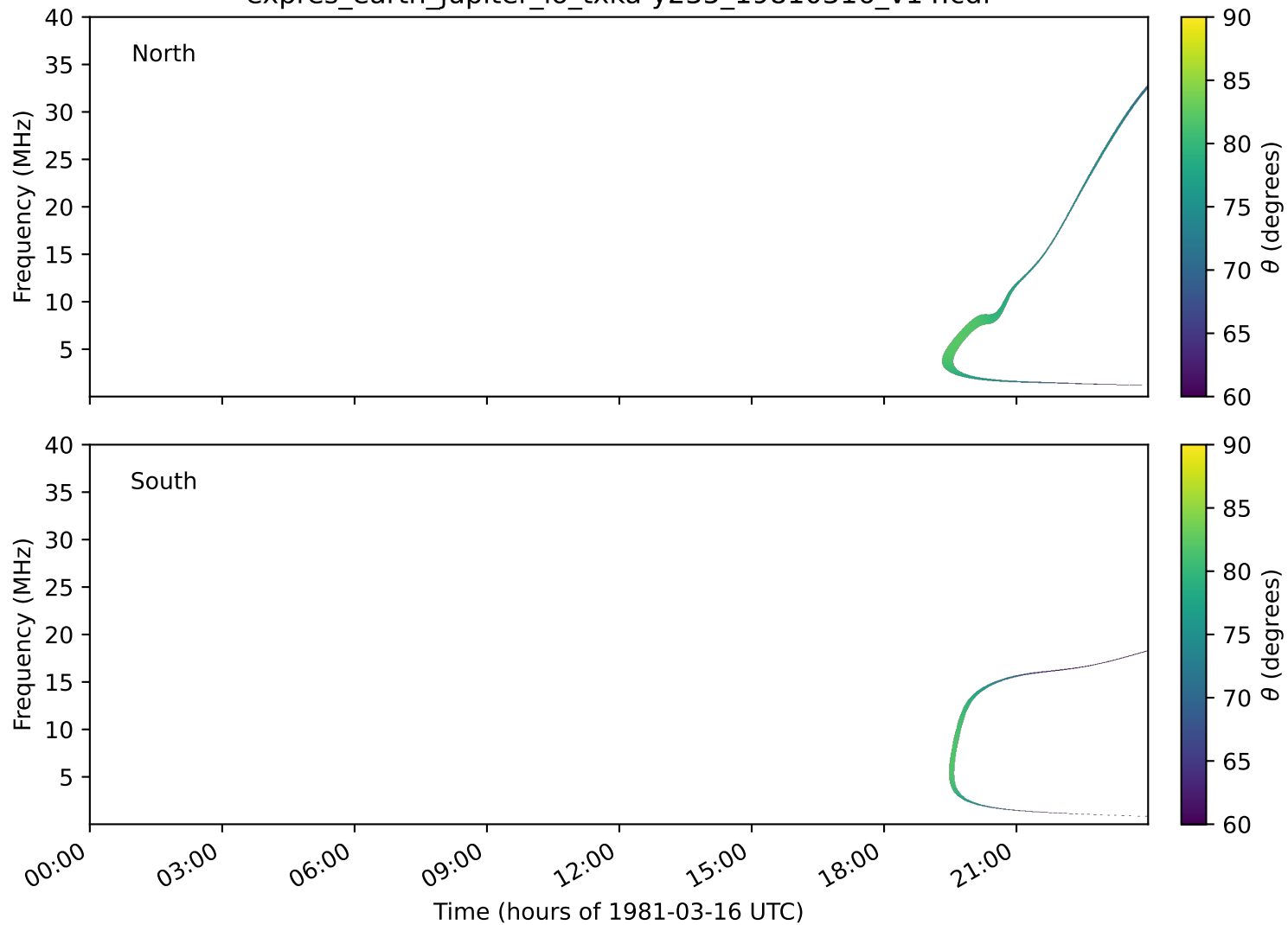
expres_earth_jupiter_io_txka-y235_19810316_v14.cdf
