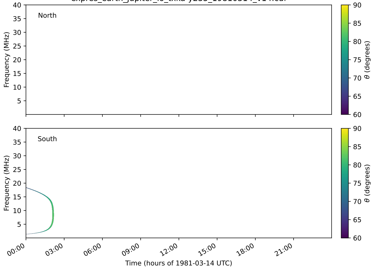
expres_earth_jupiter_io_txka-y235_19810314_v14.cdf
