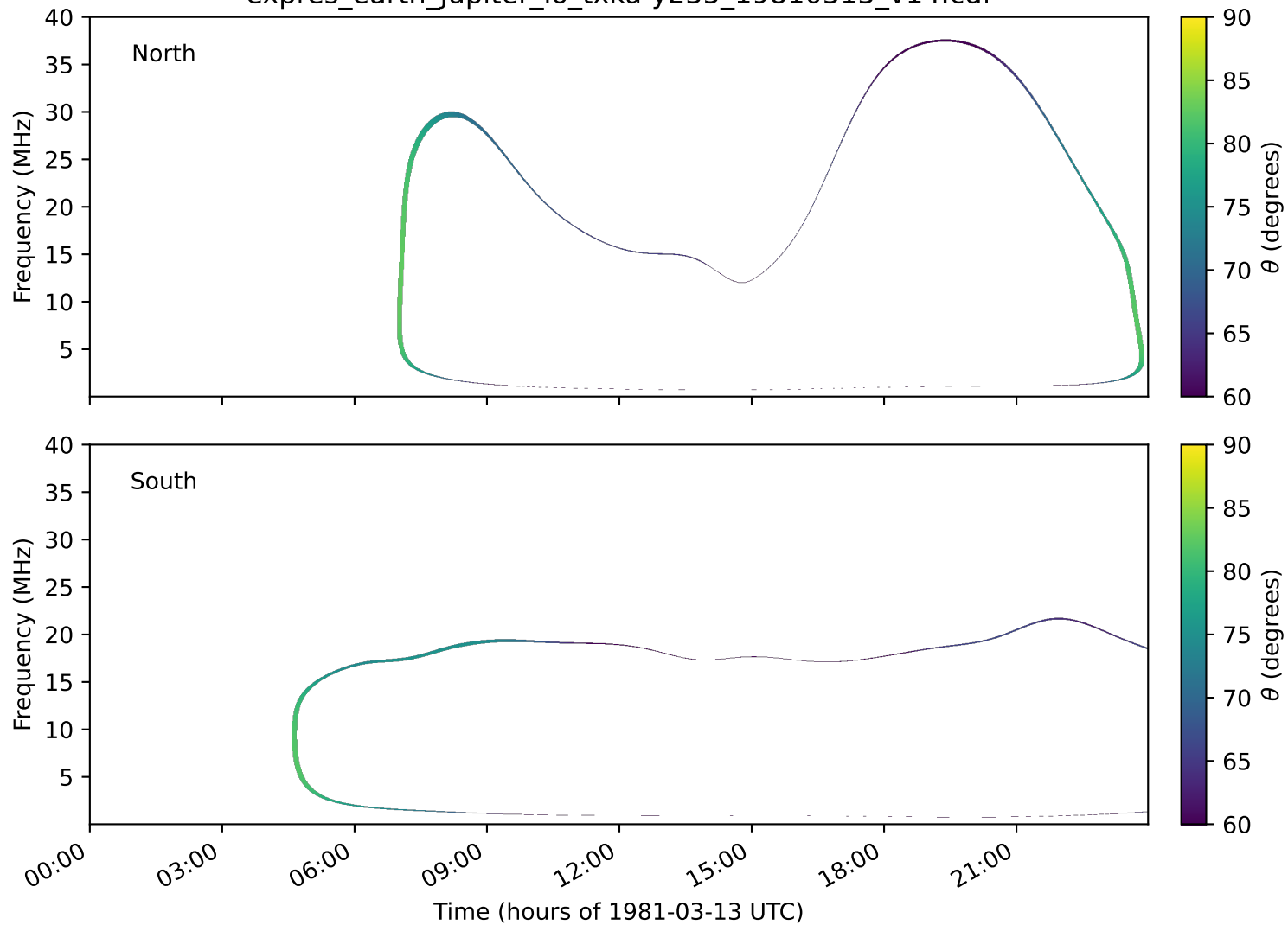
expres_earth_jupiter_io_txka-y235_19810313_v14.cdf
