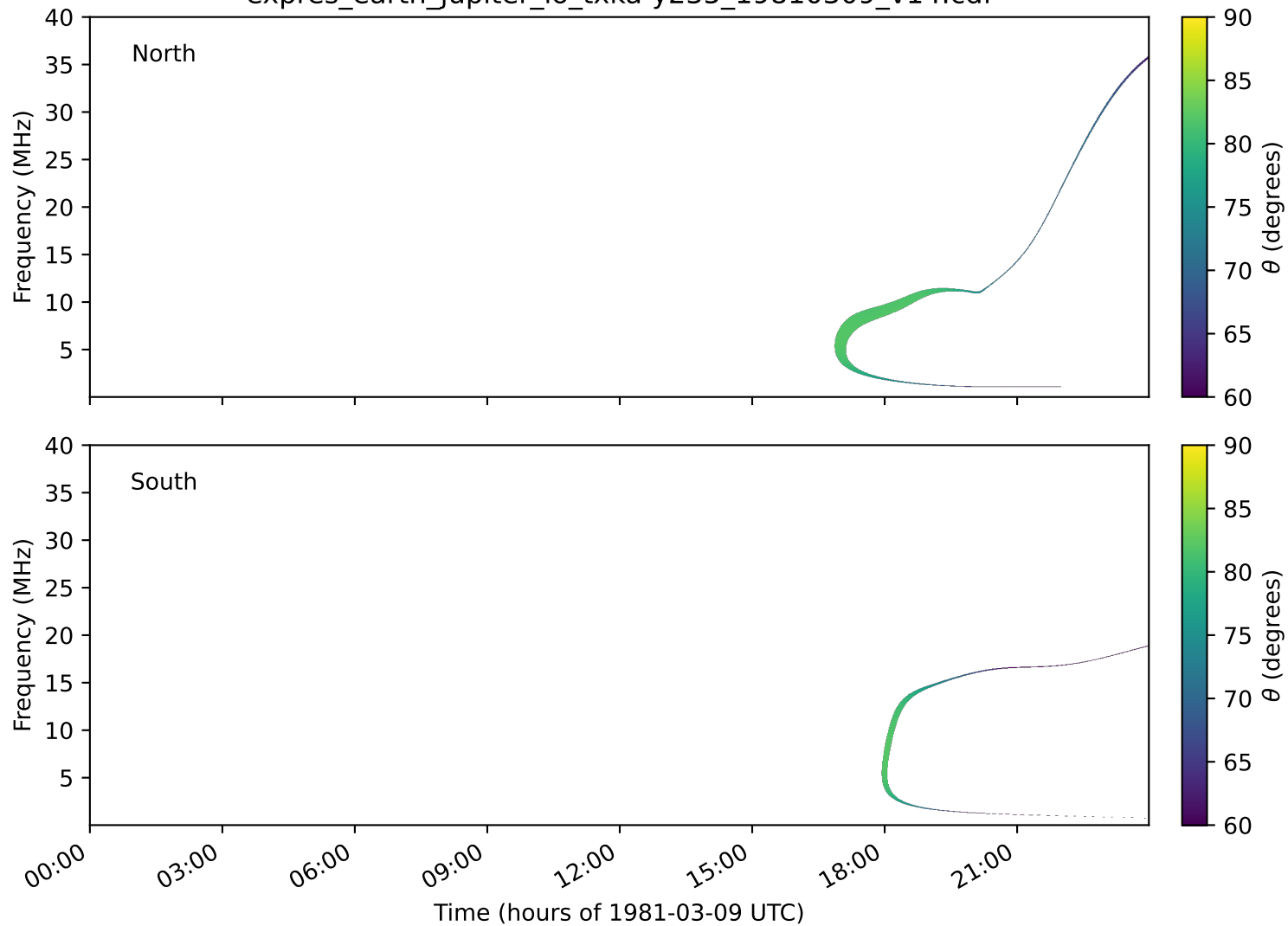
expres_earth_jupiter_io_txka-y235_19810309_v14.cdf
