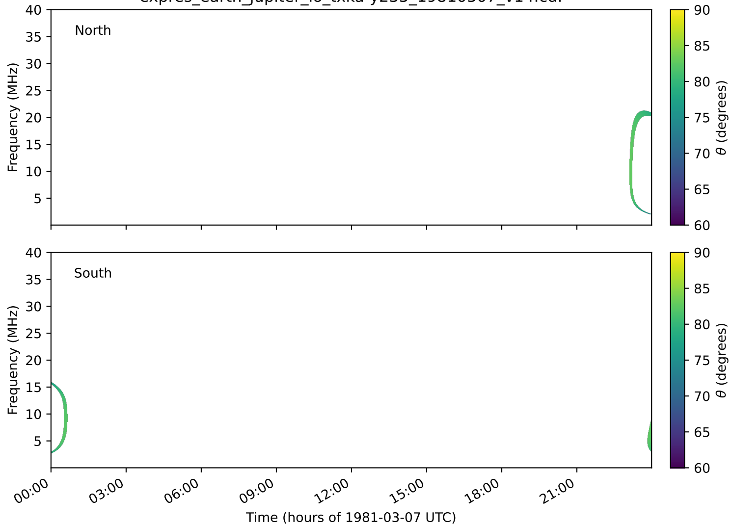
expres_earth_jupiter_io_txka-y235_19810307_v14.cdf
