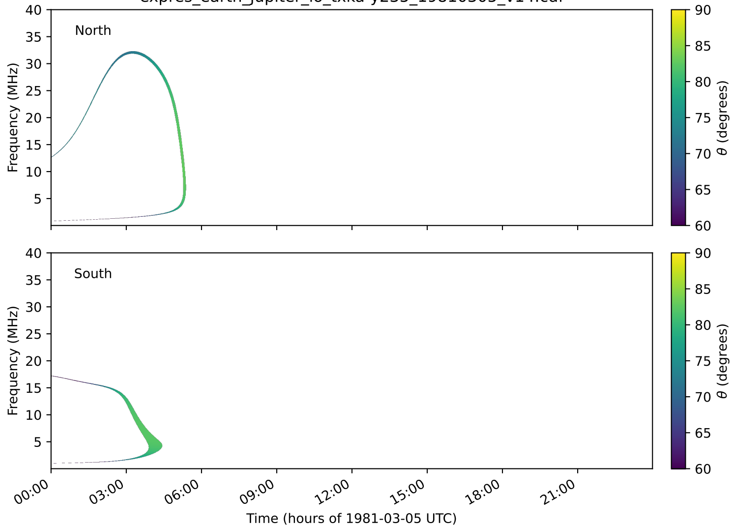
expres_earth_jupiter_io_txka-y235_19810305_v14.cdf
