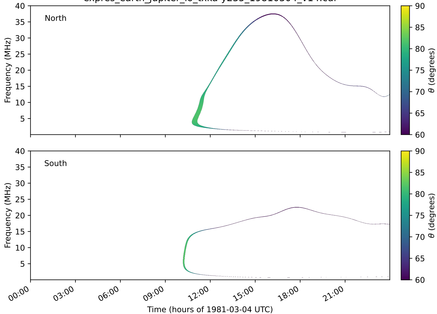
expres_earth_jupiter_io_txka-y235_19810304_v14.cdf
