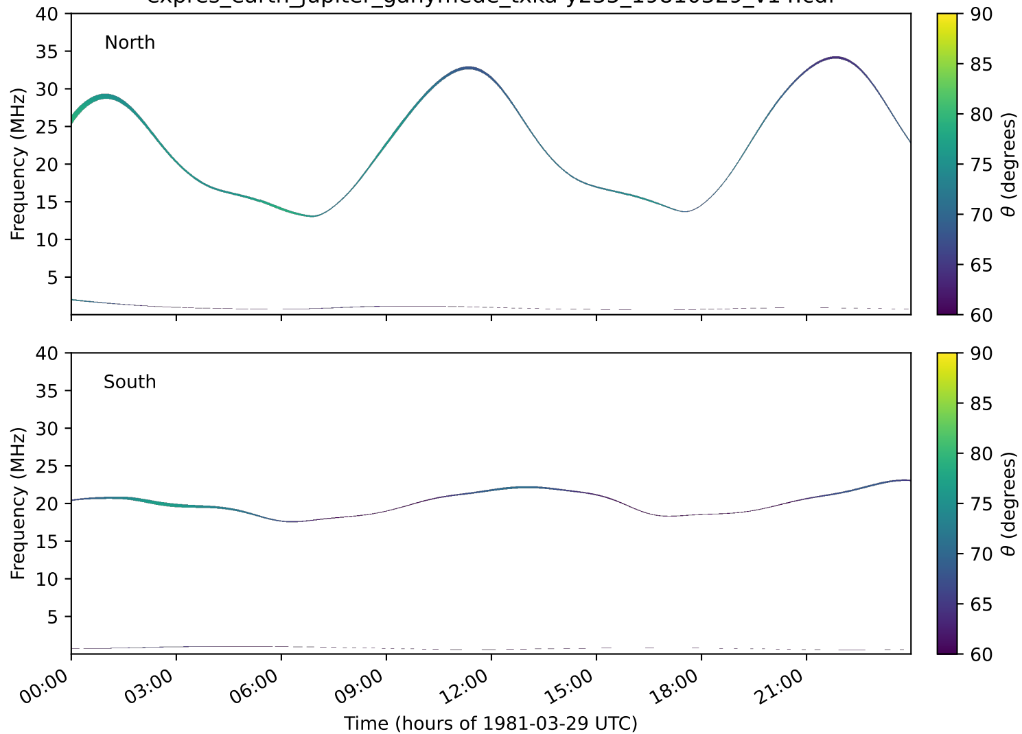
expres_earth_jupiter_ganymede_txka-y235_19810329_v14.cdf
