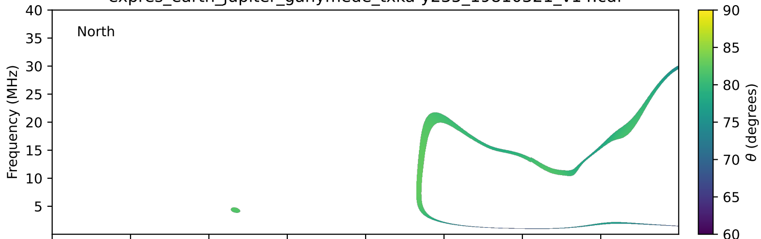
expres_earth_jupiter_ganymede_txka-y235_19810321_v14.cdf
