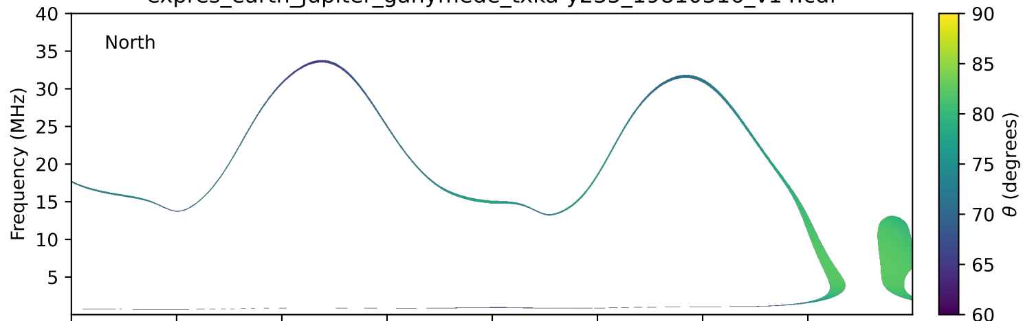
expres_earth_jupiter_ganymede_txka-y235_19810316_v14.cdf
