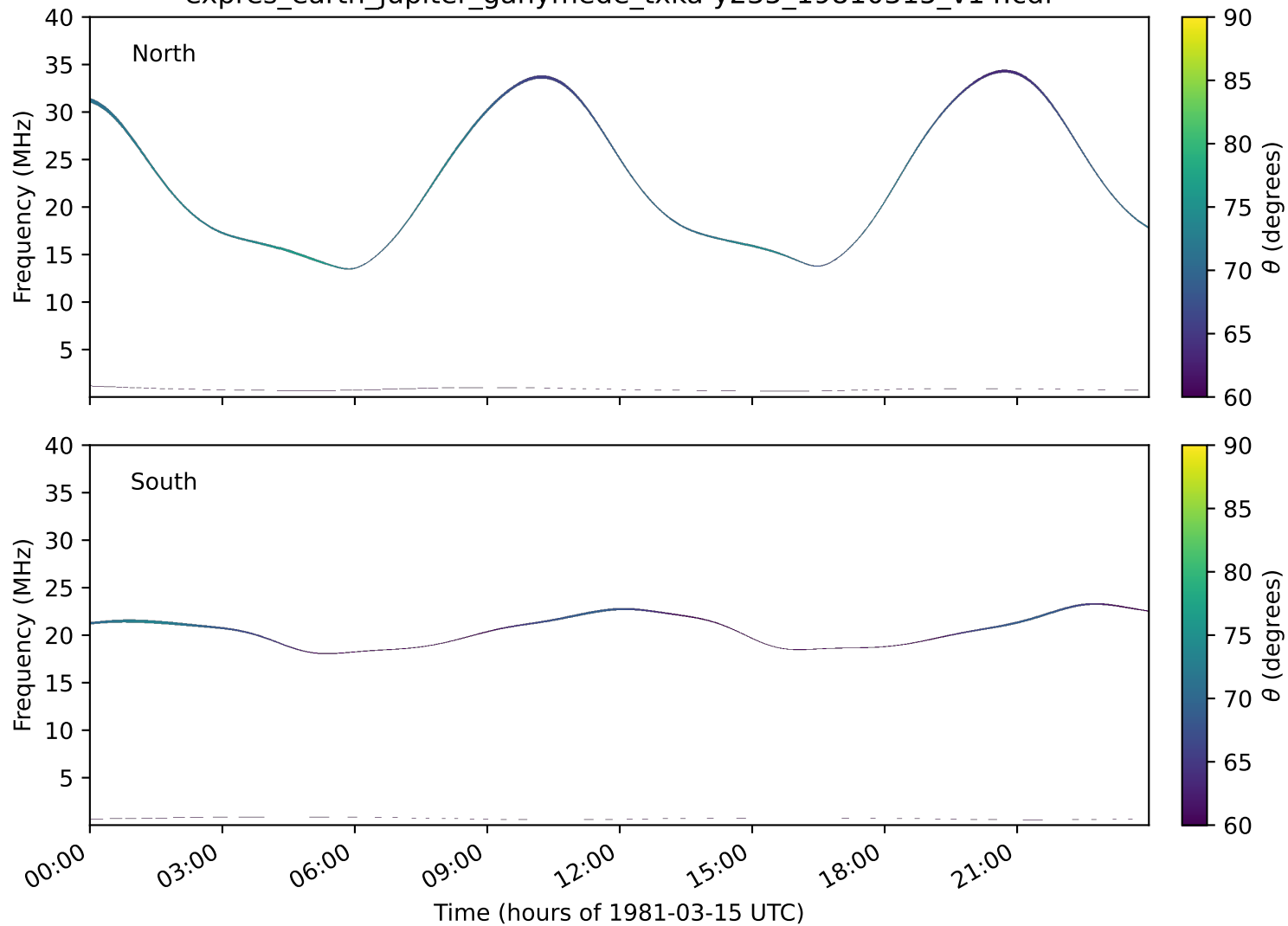
expres_earth_jupiter_ganymede_txka-y235_19810315_v14.cdf
