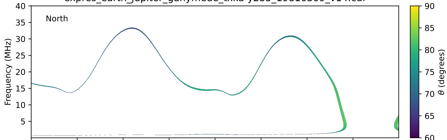
expres_earth_jupiter_ganymede_txka-y235_19810309_v14.cdf
