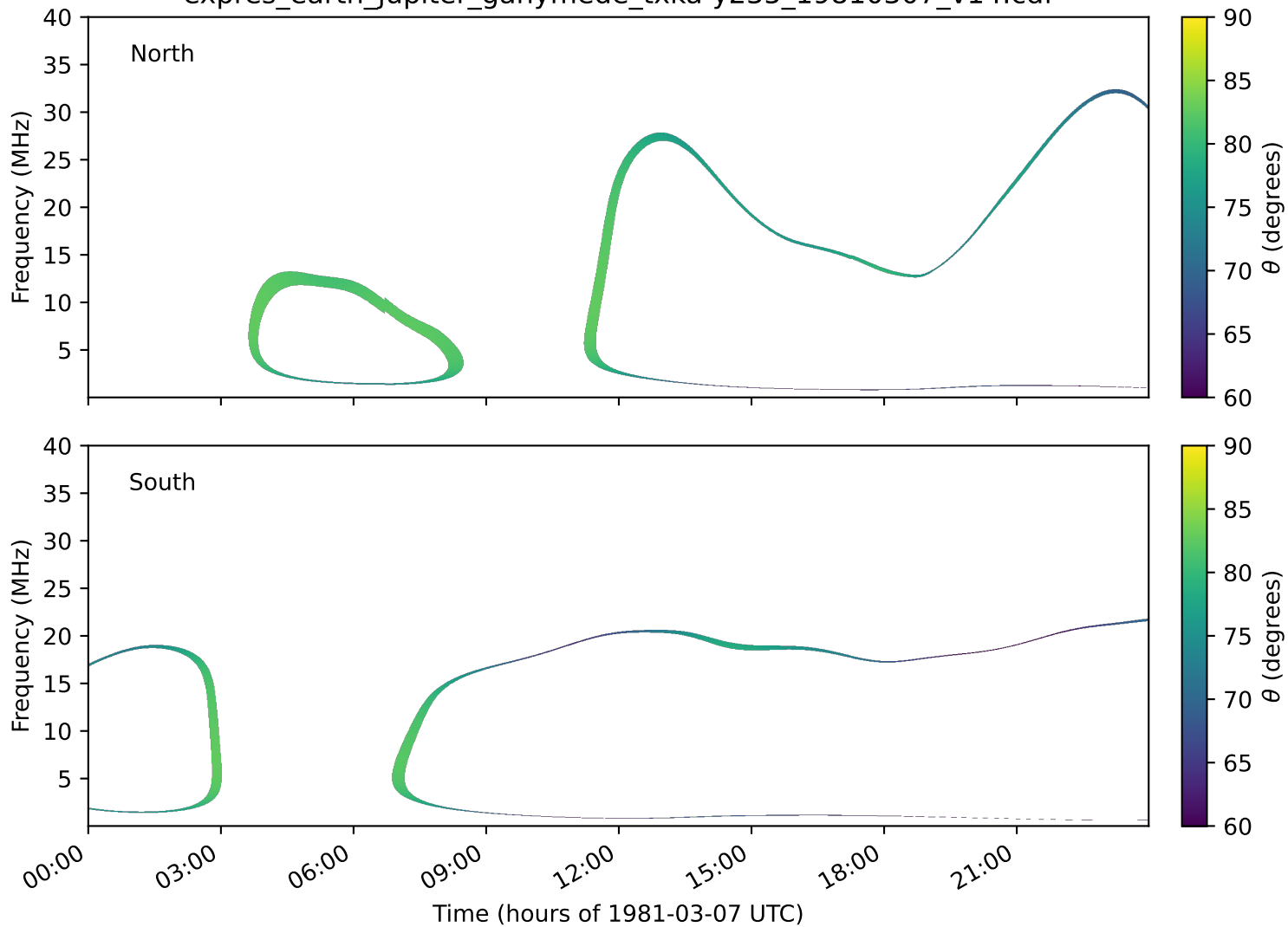
expres_earth_jupiter_ganymede_txka-y235_19810307_v14.cdf
