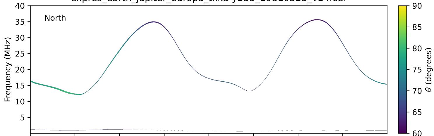
expres_earth_jupiter_europa_txka-y235_19810325_v14.cdf
