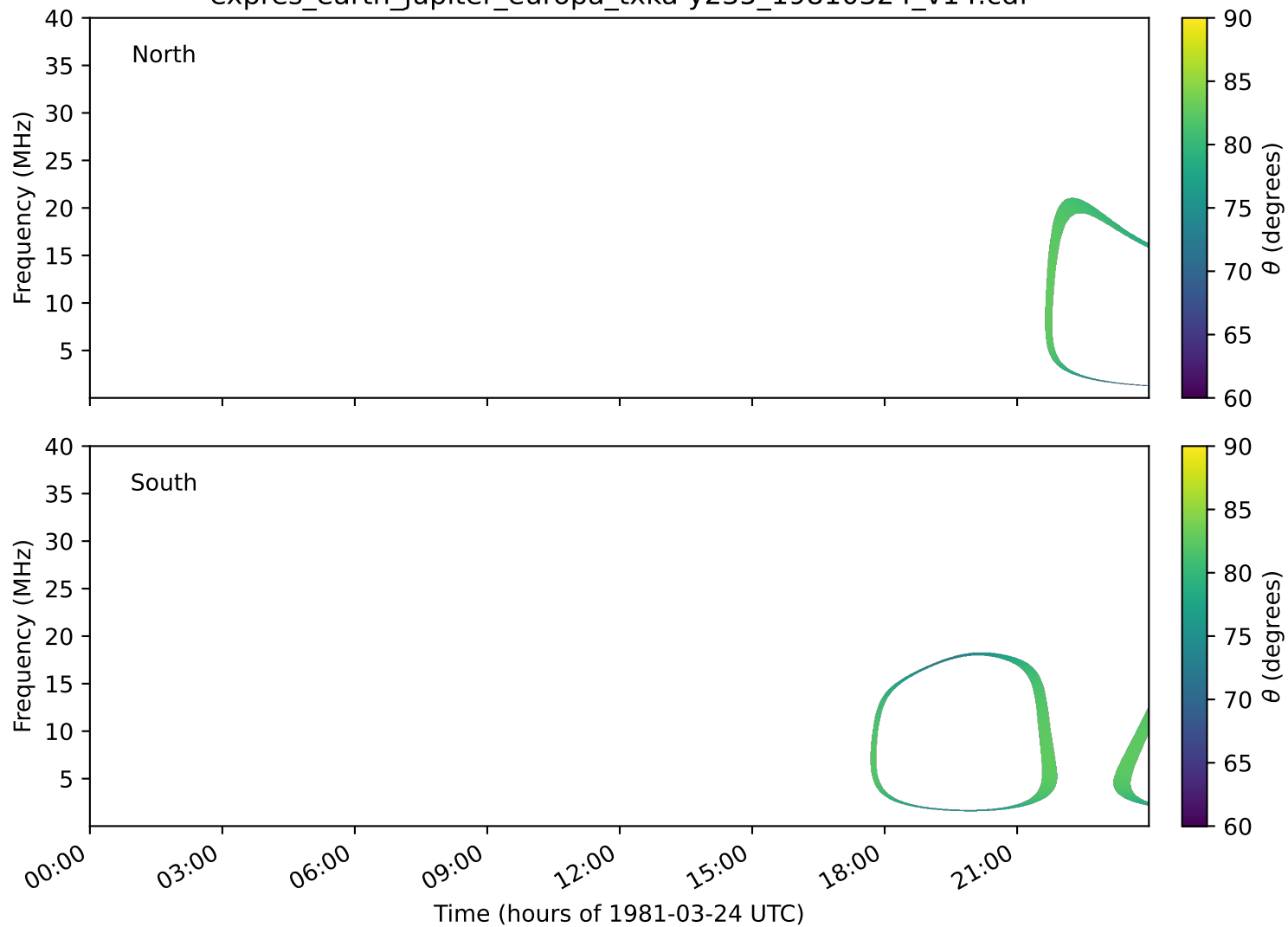
expres_earth_jupiter_europa_txka-y235_19810324_v14.cdf
