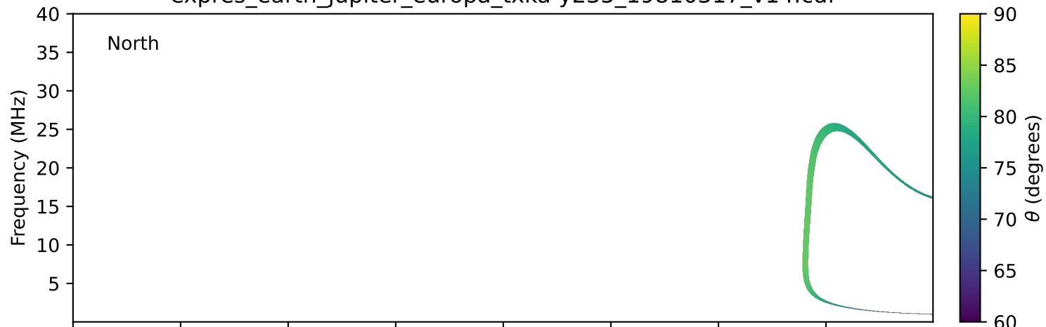
expres_earth_jupiter_europa_txka-y235_19810317_v14.cdf
