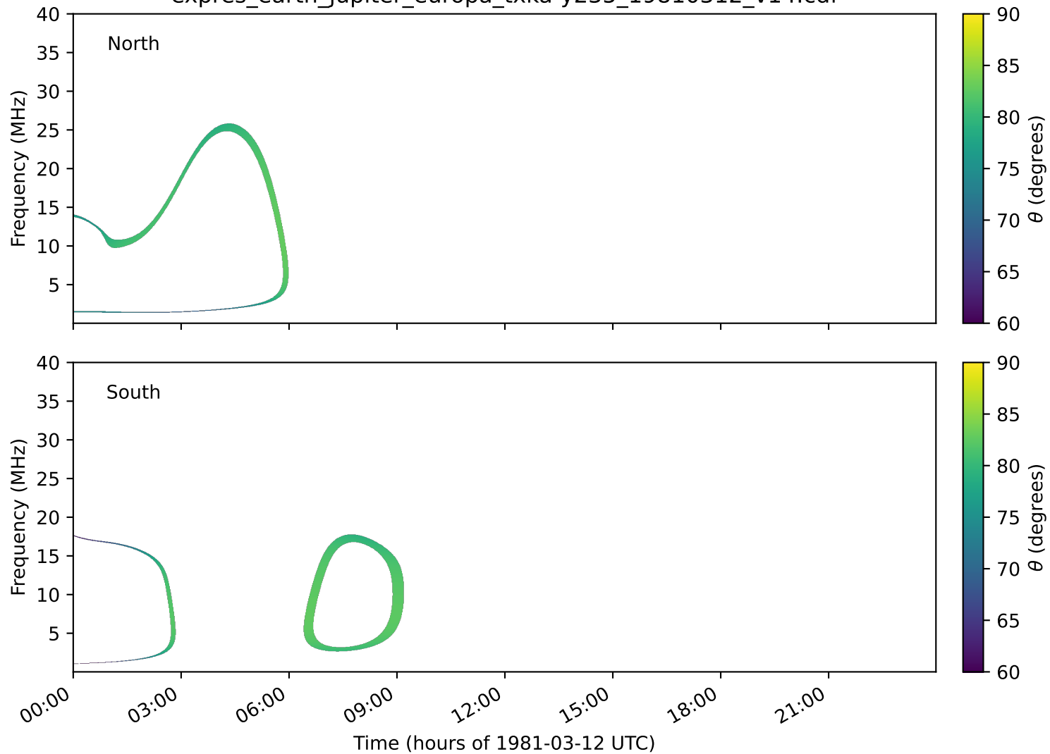
expres_earth_jupiter_europa_txka-y235_19810312_v14.cdf
