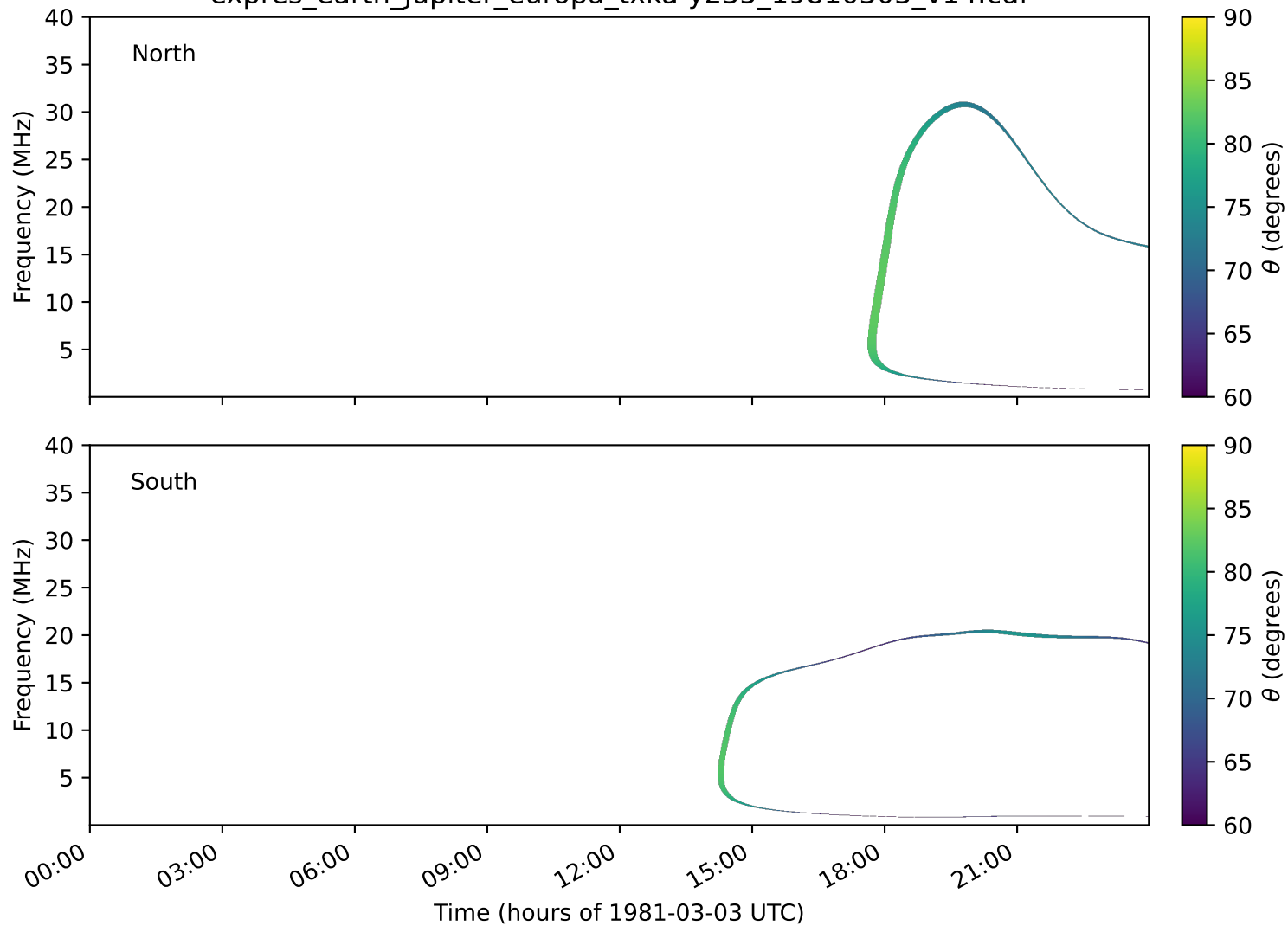
expres_earth_jupiter_europa_txka-y235_19810303_v14.cdf
