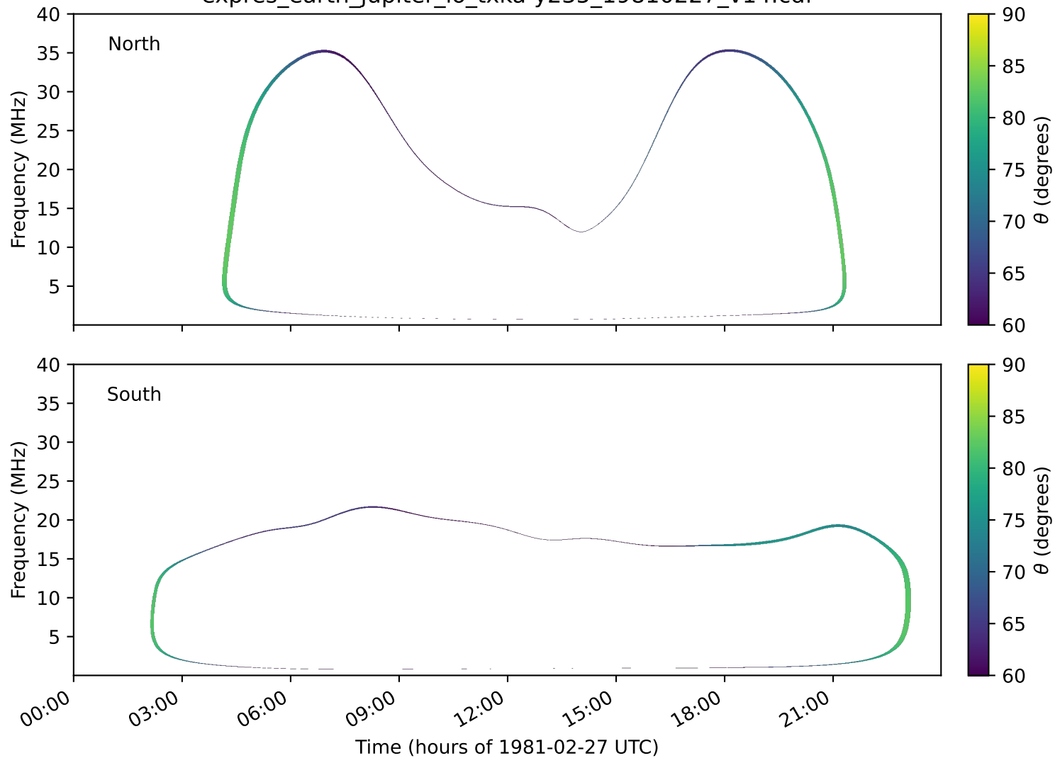
expres_earth_jupiter_io_txka-y235_19810227_v14.cdf
