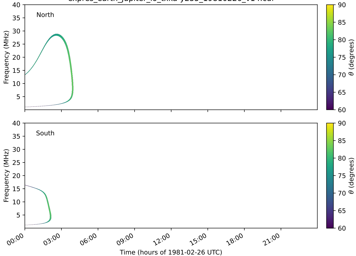
expres_earth_jupiter_io_txka-y235_19810226_v14.cdf
