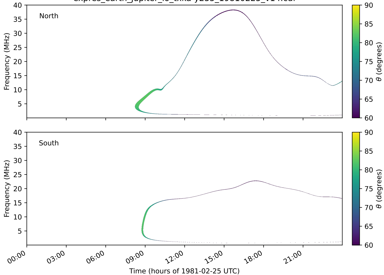
expres_earth_jupiter_io_txka-y235_19810225_v14.cdf
