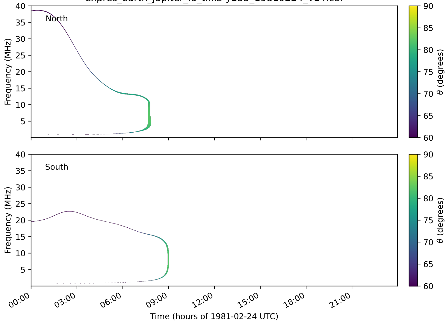
expres_earth_jupiter_io_txka-y235_19810224_v14.cdf
