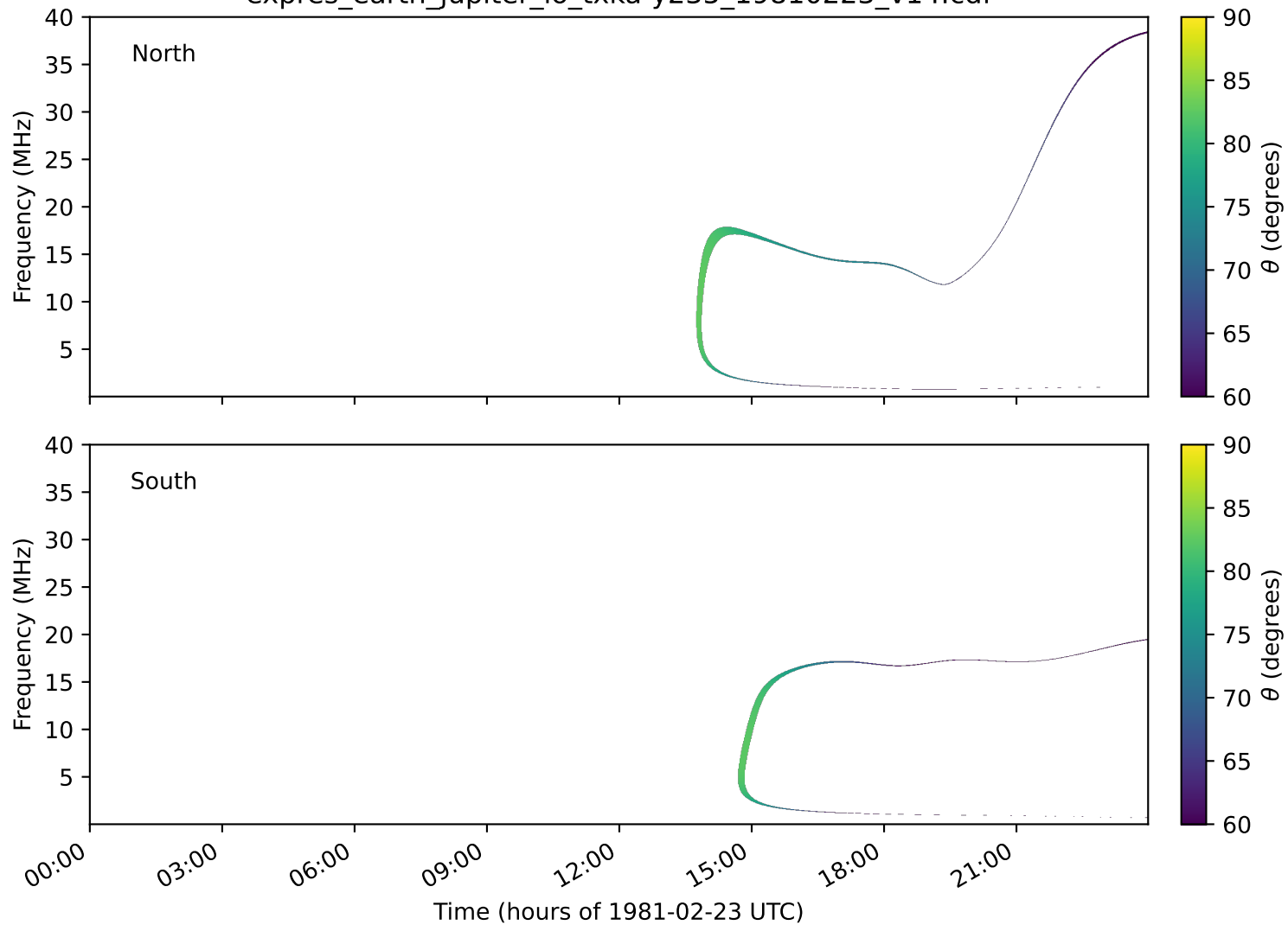
expres_earth_jupiter_io_txka-y235_19810223_v14.cdf
