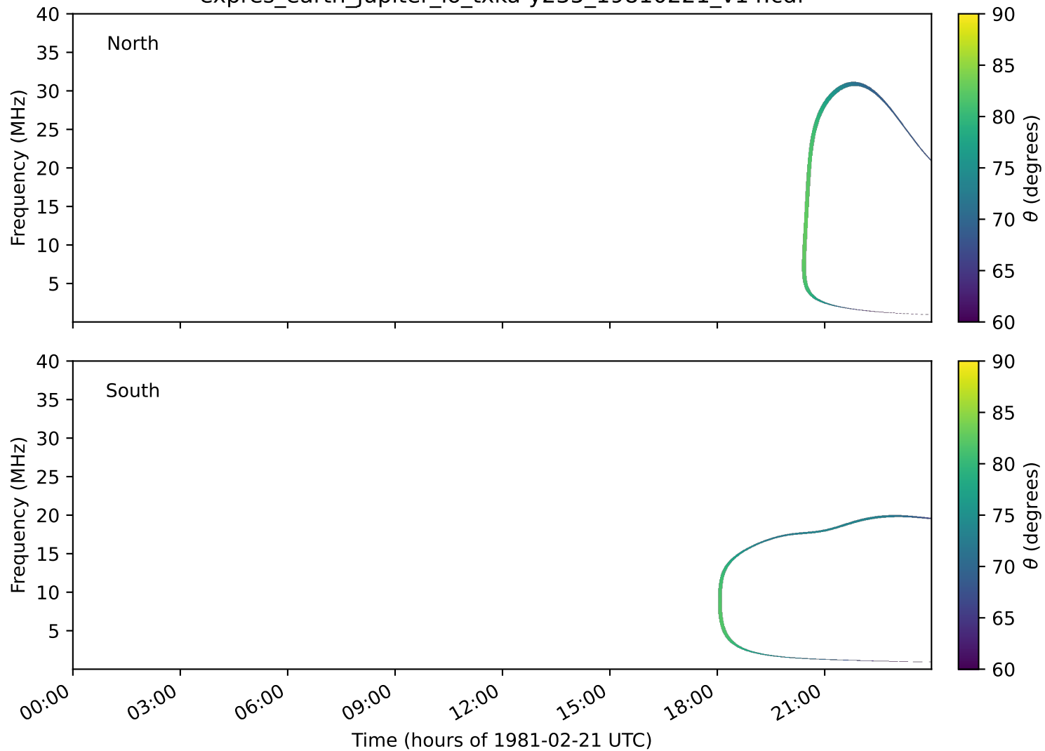
expres_earth_jupiter_io_txka-y235_19810221_v14.cdf
