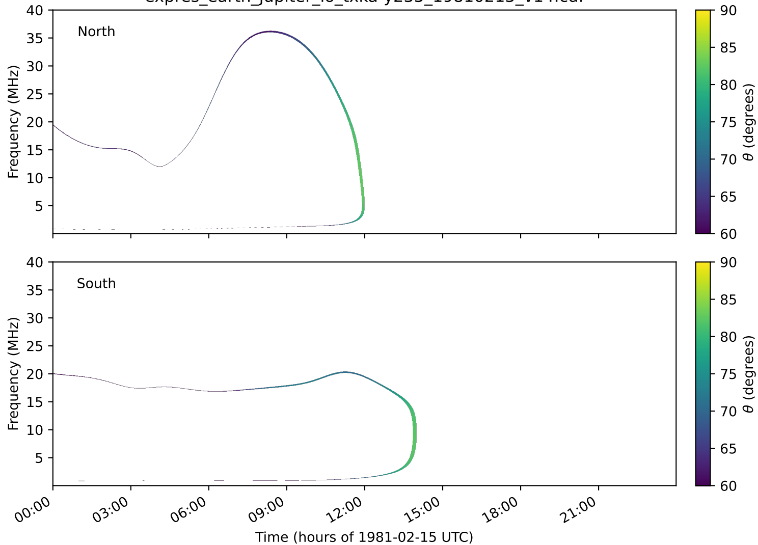
expres_earth_jupiter_io_txka-y235_19810215_v14.cdf
