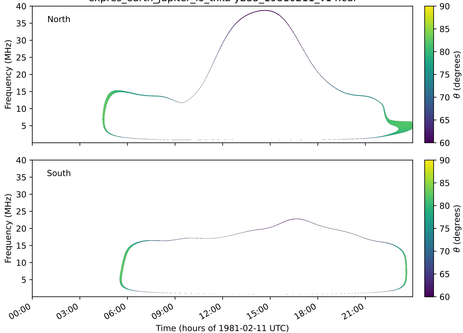
expres_earth_jupiter_io_txka-y235_19810211_v14.cdf
