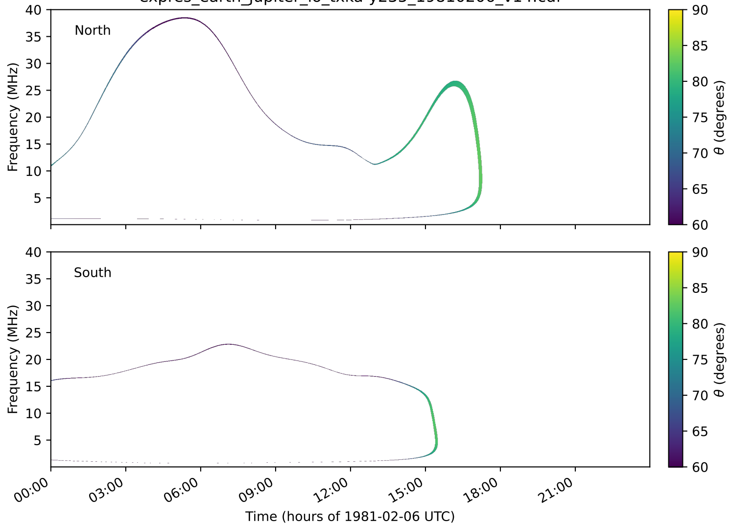
expres_earth_jupiter_io_txka-y235_19810206_v14.cdf
