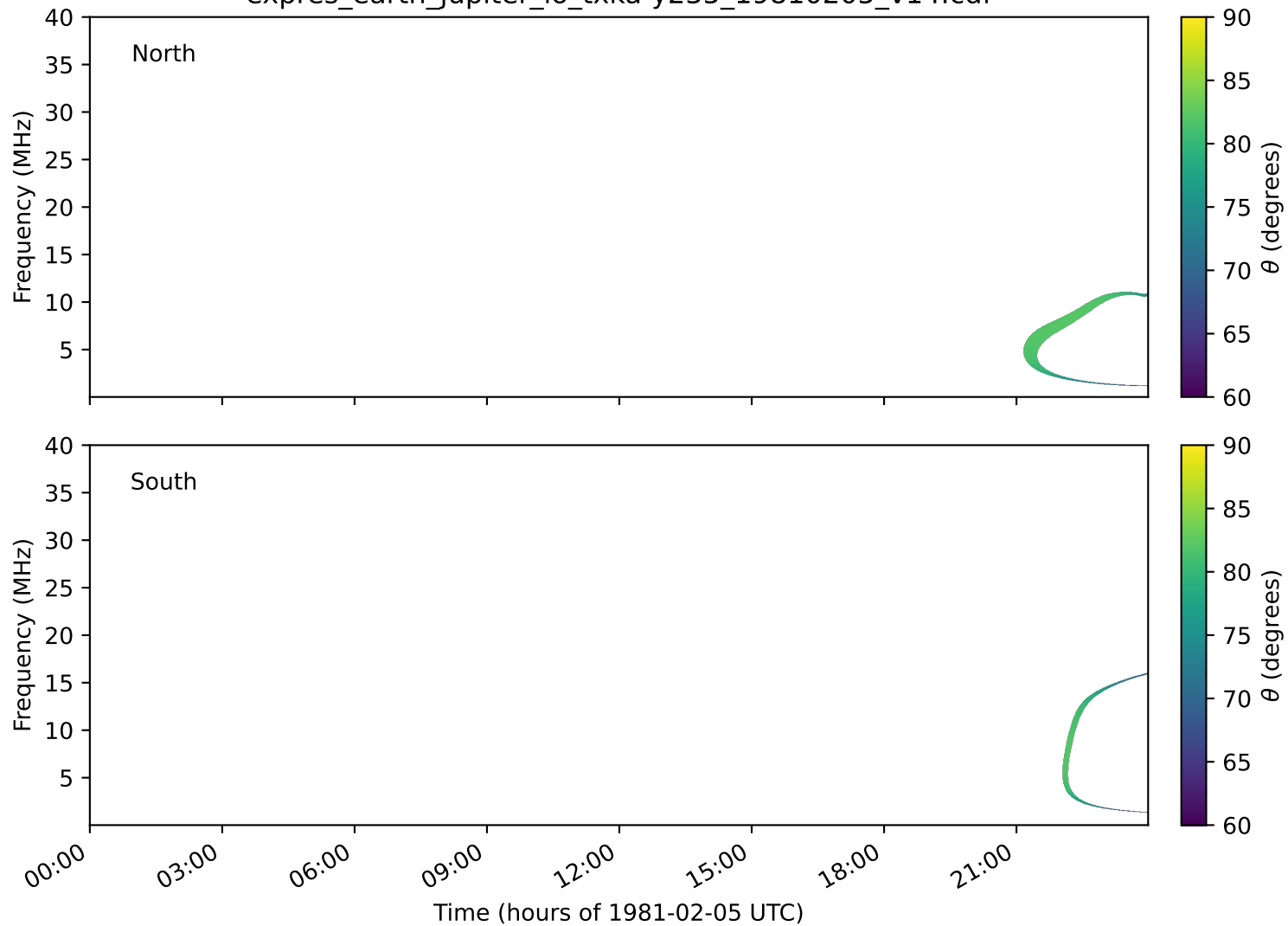
expres_earth_jupiter_io_txka-y235_19810205_v14.cdf
