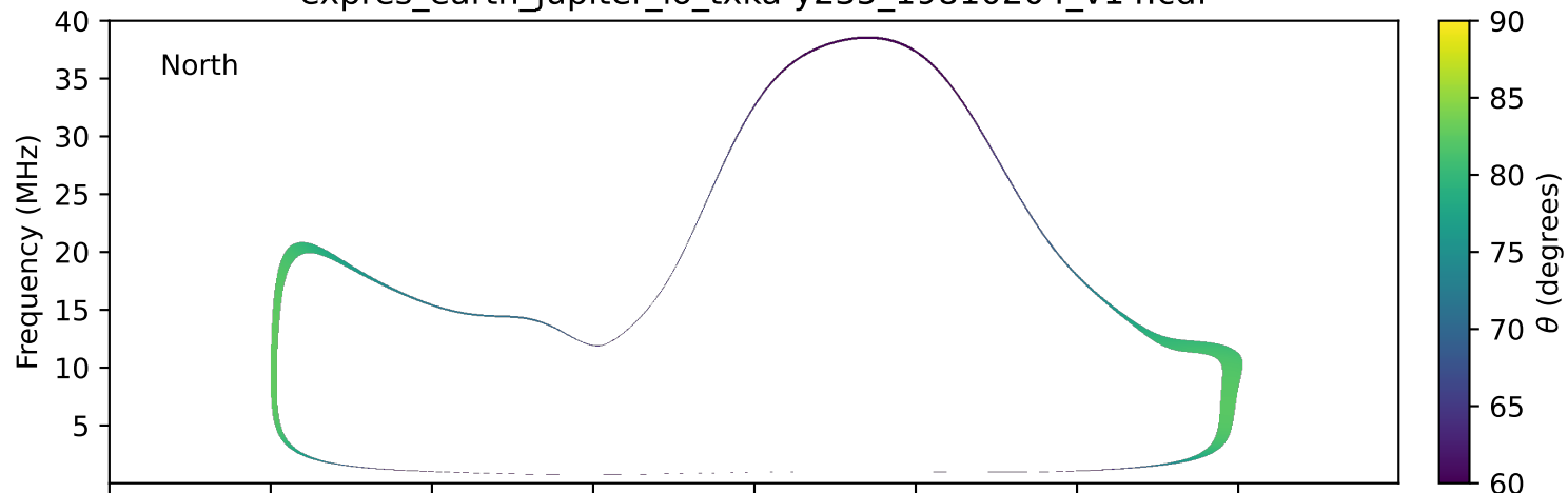
expres_earth_jupiter_io_txka-y235_19810204_v14.cdf
