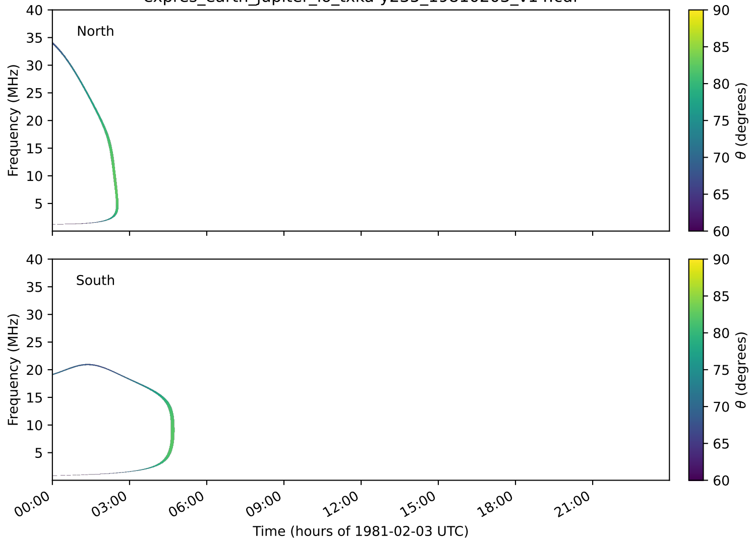
expres_earth_jupiter_io_txka-y235_19810203_v14.cdf
